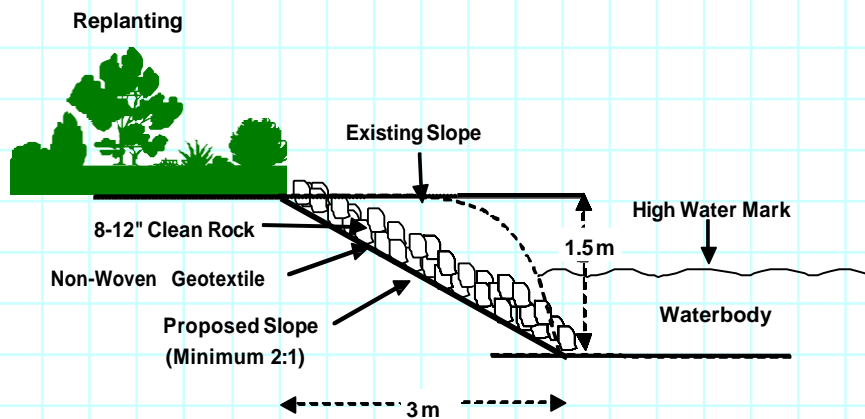
Cross-Section - Alteration to Waterway E.g. Rip Rap Erosion Control at Shoreline
